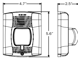
Wall-mount horn/strobes
