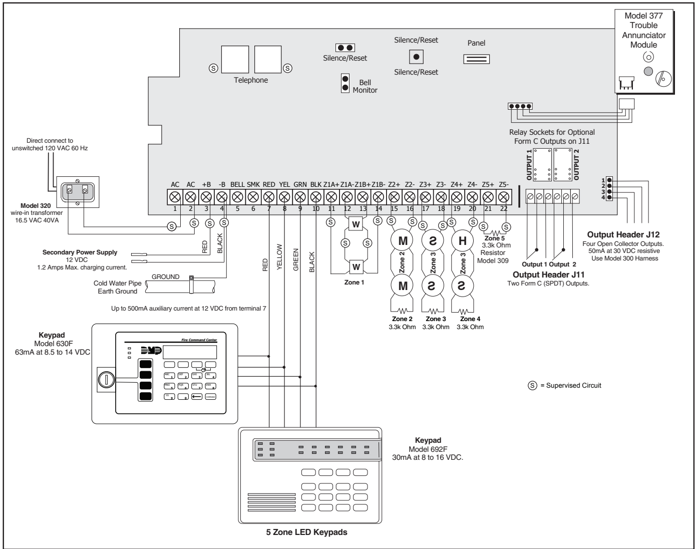
XR5FC System Configuration Diagram
